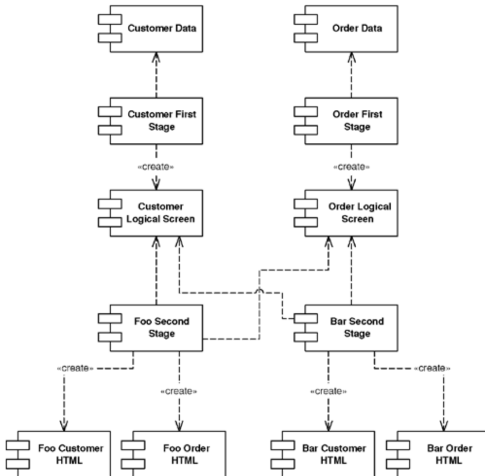
Figure 14.9. Two-stage view with two appearances.
