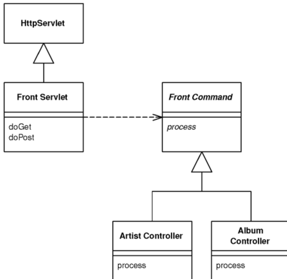
Figure 14.3. The classes that implement Front Controller.
