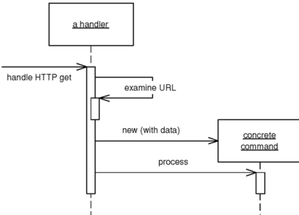
Figure 14.2. How the Front Controller works.
