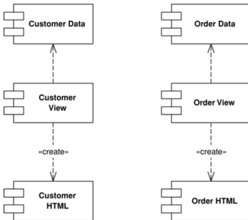
Figure 4.2. A single-stage view.
