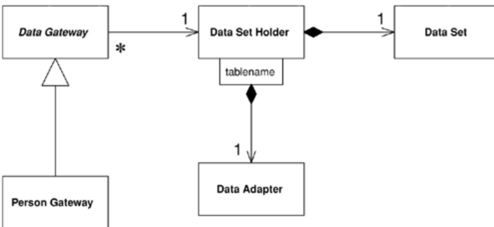
Figure 10.1. Class diagram of data-set-oriented gateway and the supporting data holder.
