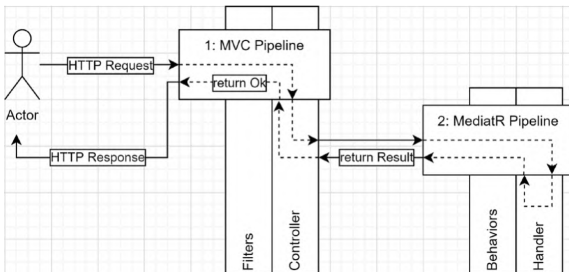
Figure 15.8: High-level flow of a successful HTTP request
