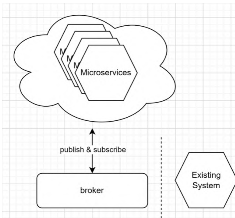
Figure 16.27: A microservices system that interacts with an event broker and an existing system that is disconnected from the microservices
