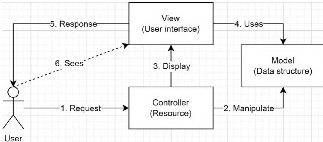
Figure 4.1: MVC workflow
