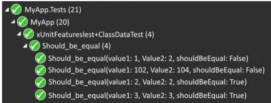
Figure 2.6: Test Explorer
