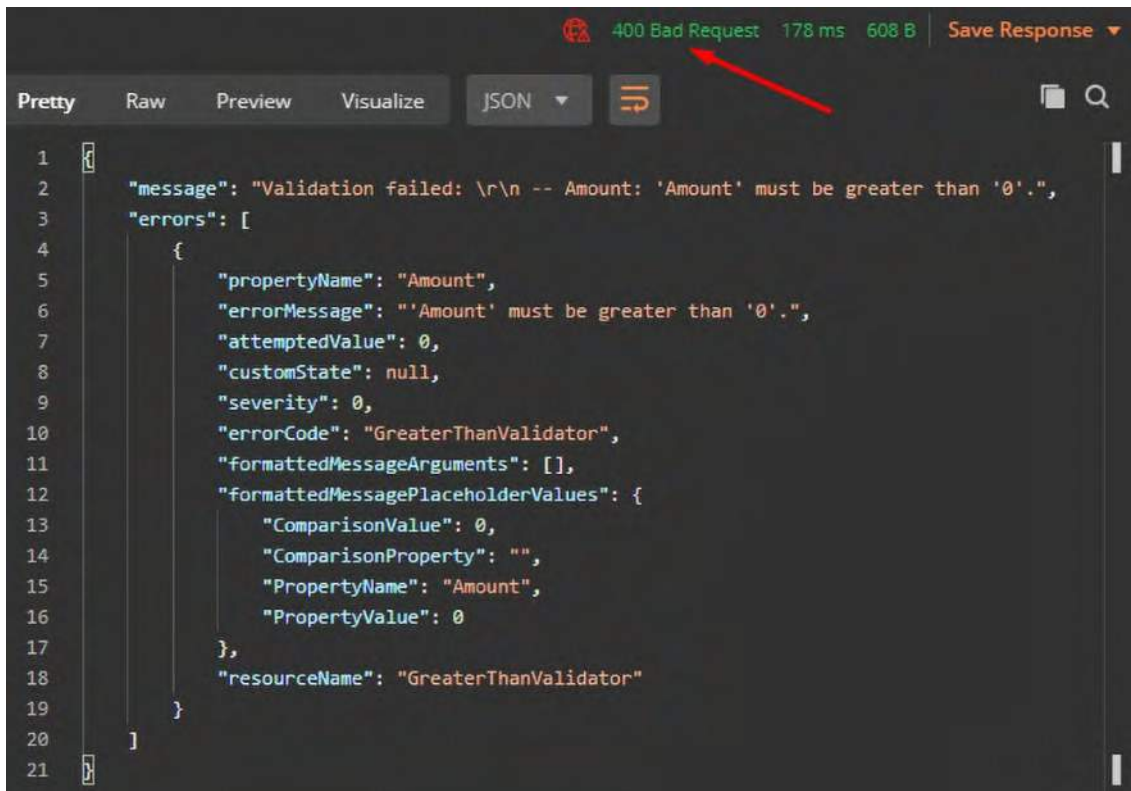
Figure 15.11: The result of ThrowFluentValidationExceptionBehavior handled by FluentValidationExceptionHandler
