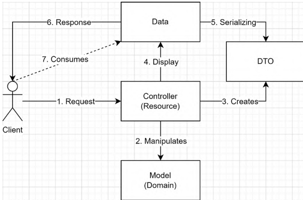
Figure 5.2: MVC workflow with a DTO
