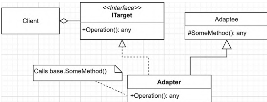
Figure 9.13: Adapter class diagram inheriting the Adaptee
