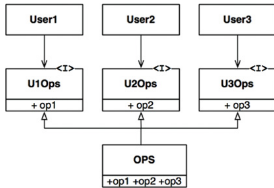
Figure 10.2 Segregated operations
