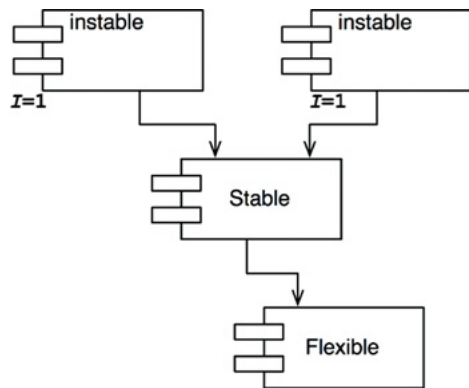
Figure 14.9 SDP violation
