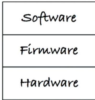
Figure 29.1 Three layers
