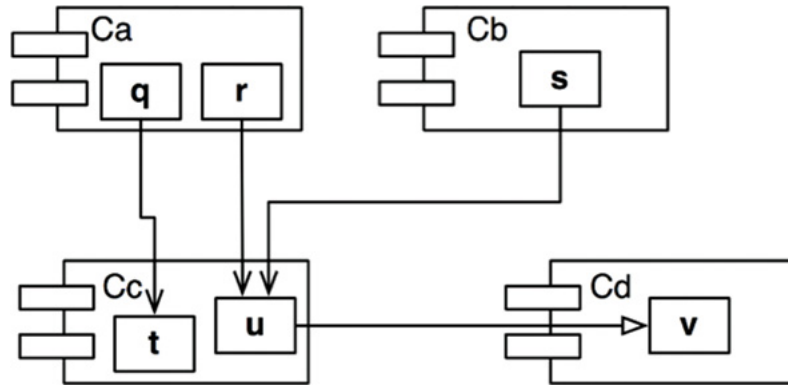
Figure 14.7 Our example
