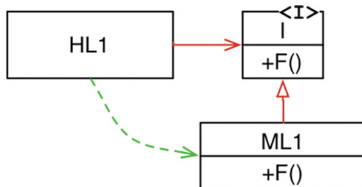
Figure 5.2 Dependency inversion
