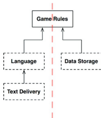
Figure 25.4 Simplified diagram
