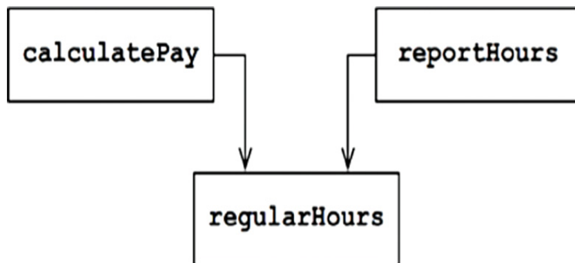
Figure 7.2 Shared algorithm
