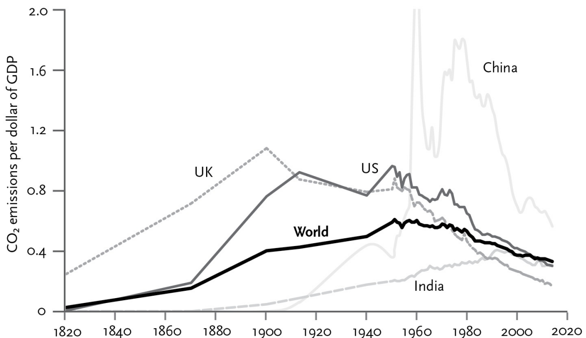
Figure 10-7: Carbon intensity ( \text{CO}_2 emissions per dollar of GDP), 1820–2014
