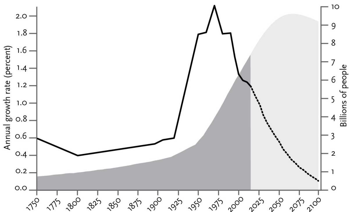
Figure 10-1: Population and population growth, 1750–2015 and projected to 2100
