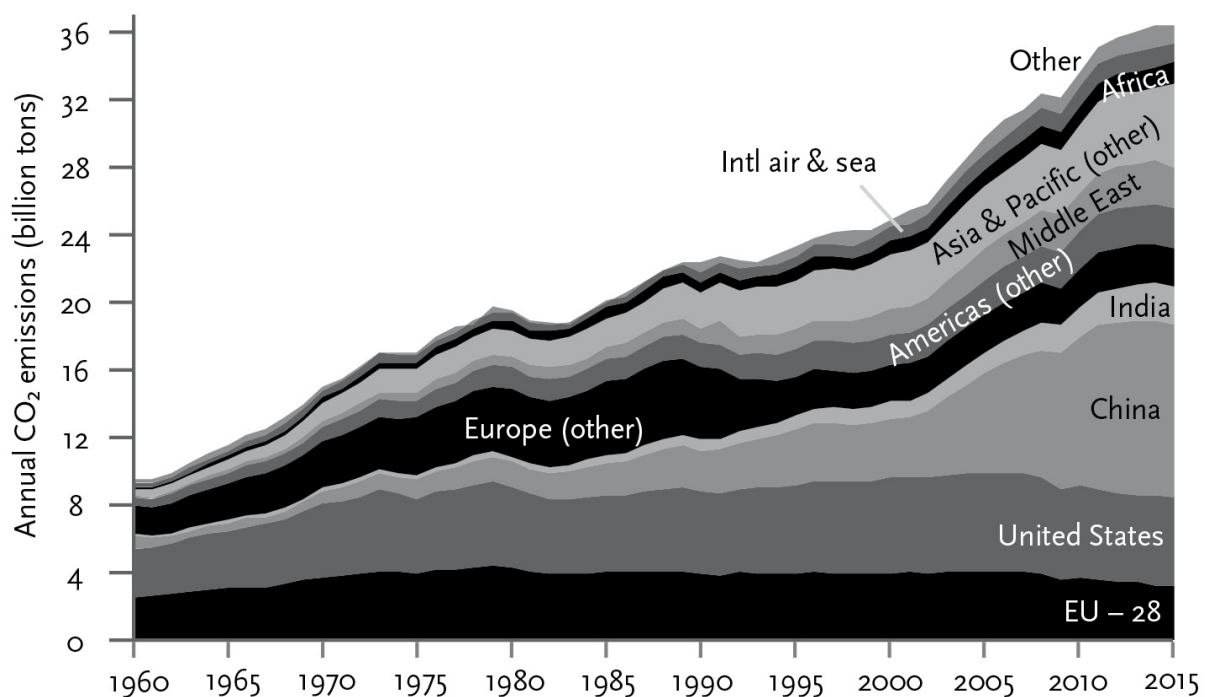
Figure 10-8: CO 2 emissions, 1960–2015
