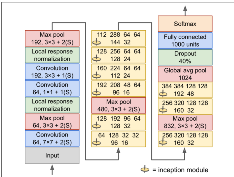
Figure 14-14. GoogLeNet architecture
