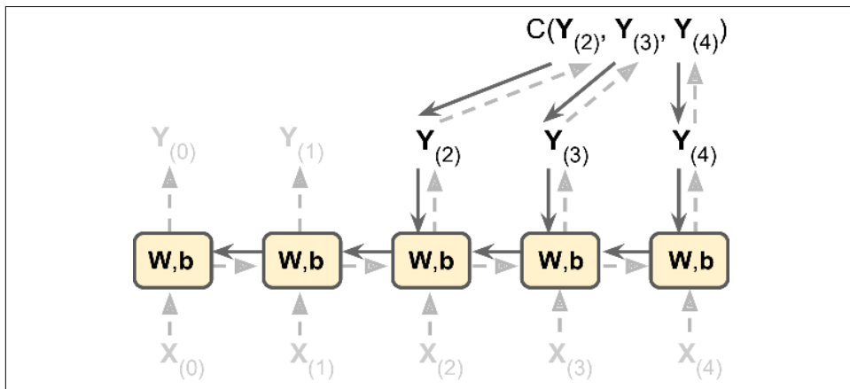
Figure 15-5. Backpropagation through time
